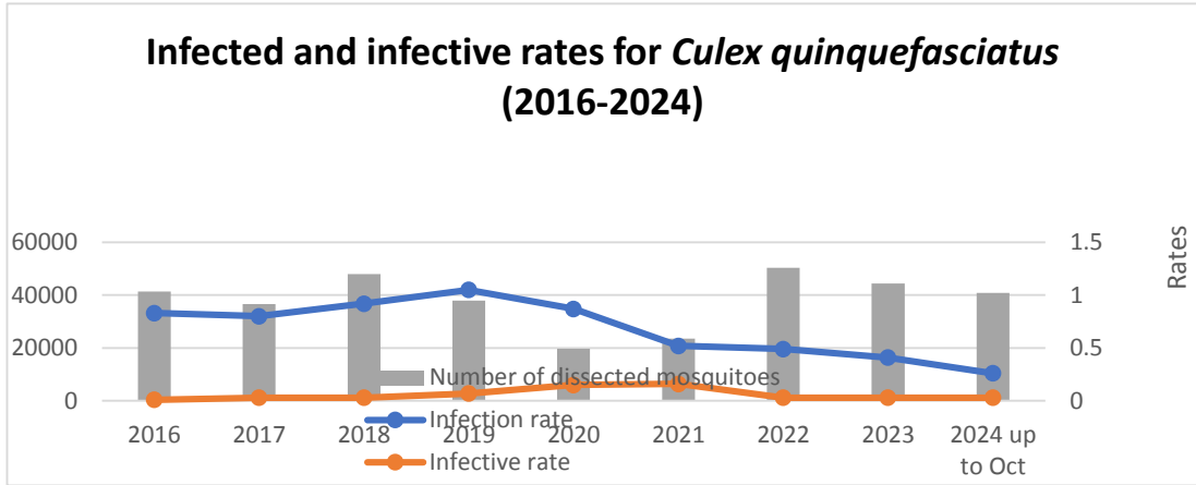
Figure 6- Infected and infective rates of mosquitoes for Culex quinquefasciatus
